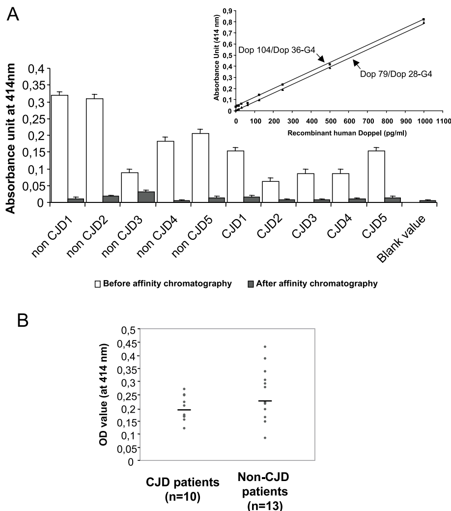
Fig. 3. A: Detection of Dpl in human brain homogenates, using a two-site immunoassay before and after depletion by affinity chromatography. Standard curves were established and the Dop79–Dop28 combination was selected for the sample assay. We used 100 \mu l of elution product, or of homogenate centrifuged for 10 min, for the immunometric assay. B: Analysis of brain homogenates from 10 CJD and 13 non-CJD patients. 100 \mu l of brain homogenates were assayed as described. Absorbance values, with the median, are represented on the graph for both series.
